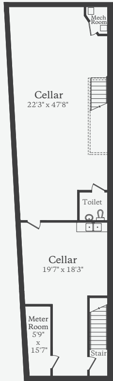
Cellar Floor
