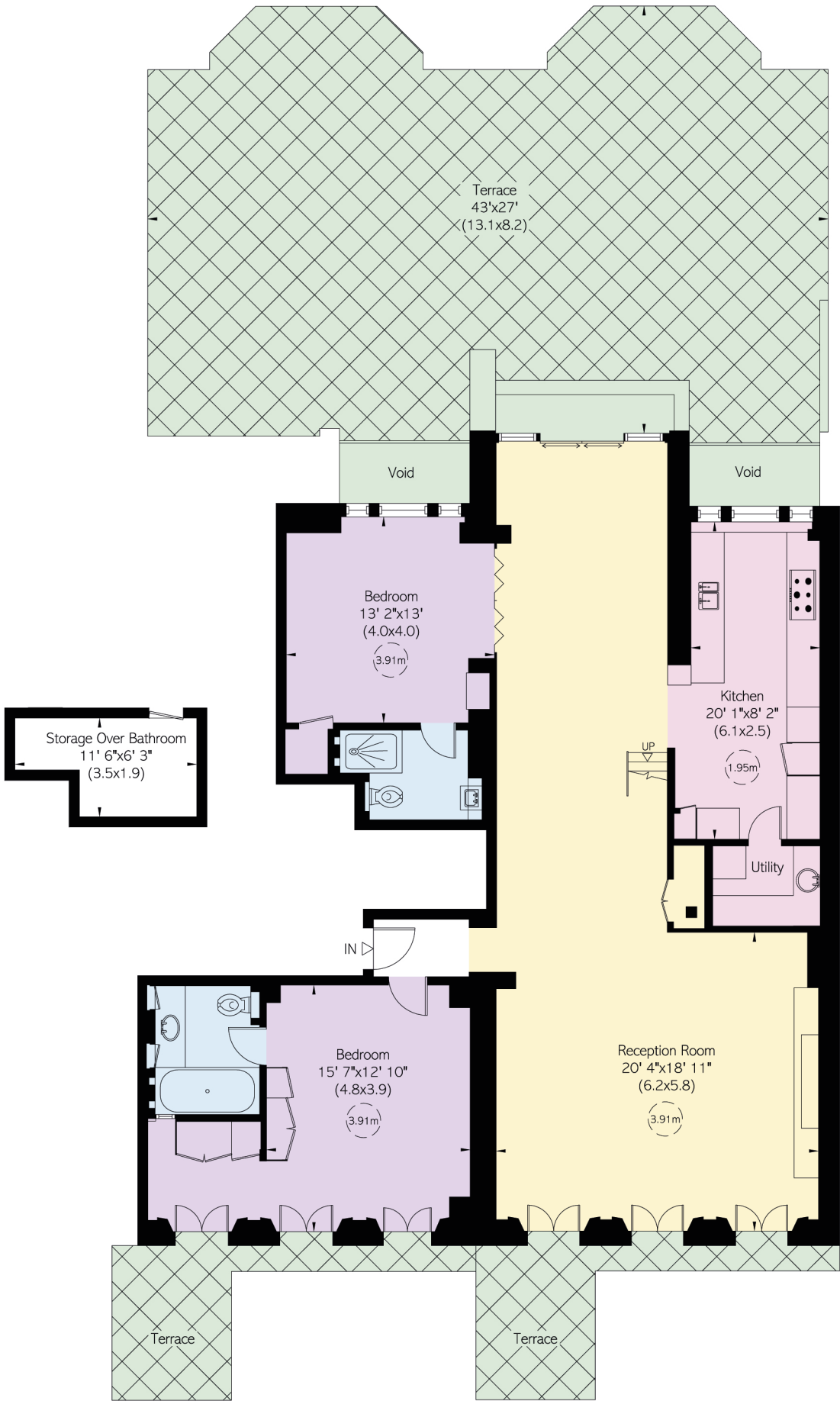
First Floor
